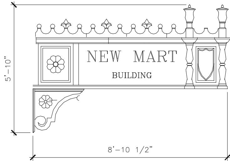
SIDE
