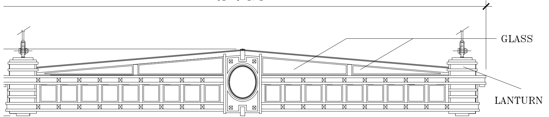
FRONT ELEVATION
