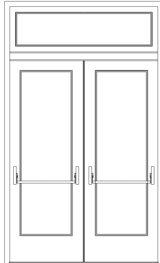
INTERIOR ELEVATION
