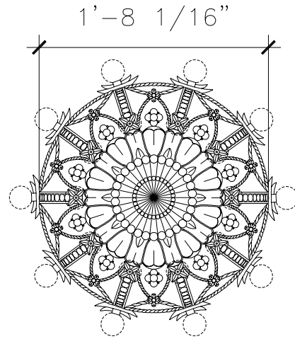
SECTION B
