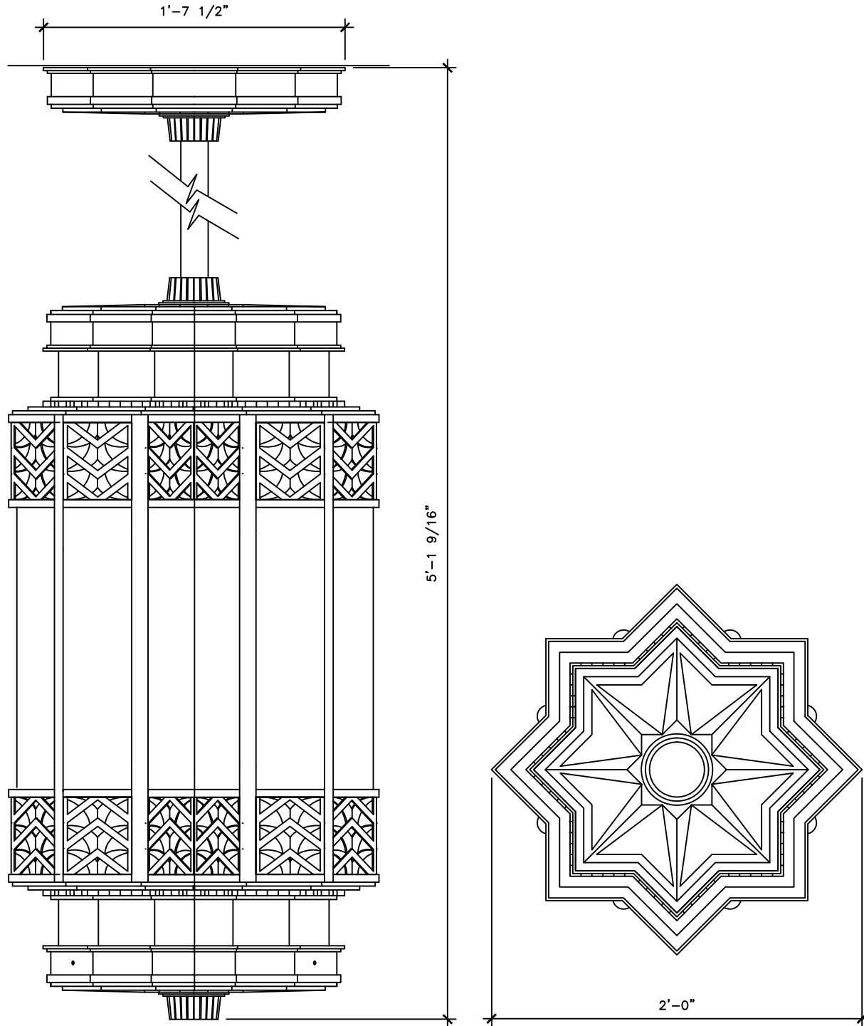
BOTTOM VIEW
