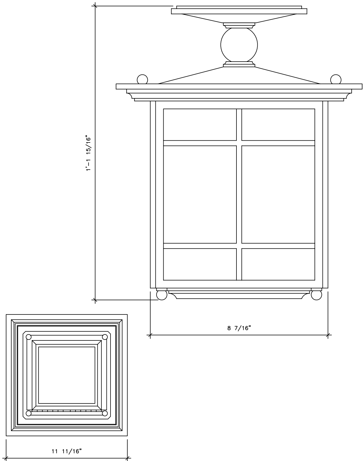
BOTTOM VIEW
